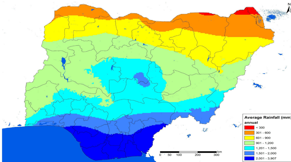
Figure 1. Average annual rainfall (1951-2000)
